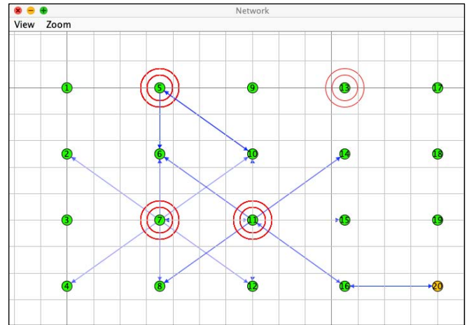
Fig. 4. Deployment of the SDWSN.
